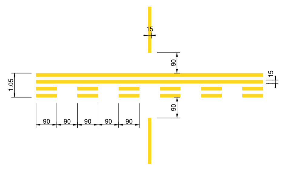
Detail ① : Holding position marking 1:100
