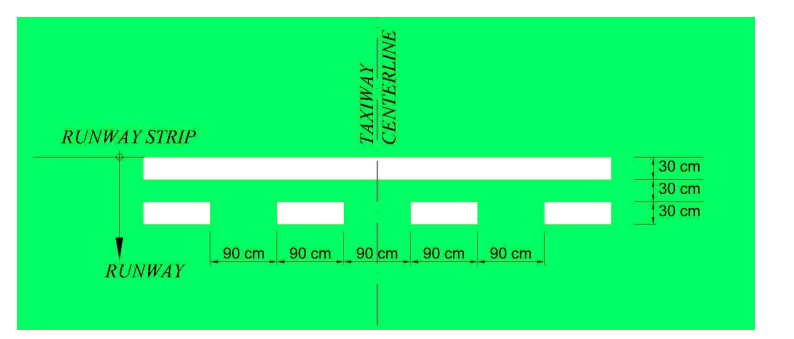
Detail ③ : Holding position marking Rollweg Gras 1:100
