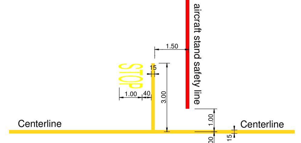
Detail ② : STOP - Marking, aircraft stand safety line 1:100
